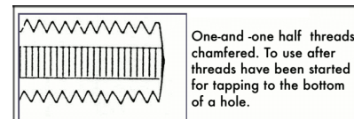
Bottoming Tap
