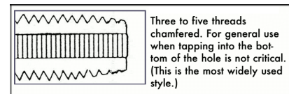
Plug Tap
